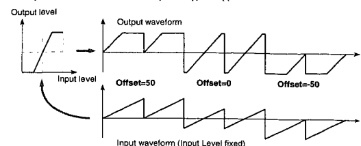
Example of when Offset is modified (Table Type: Clip)
