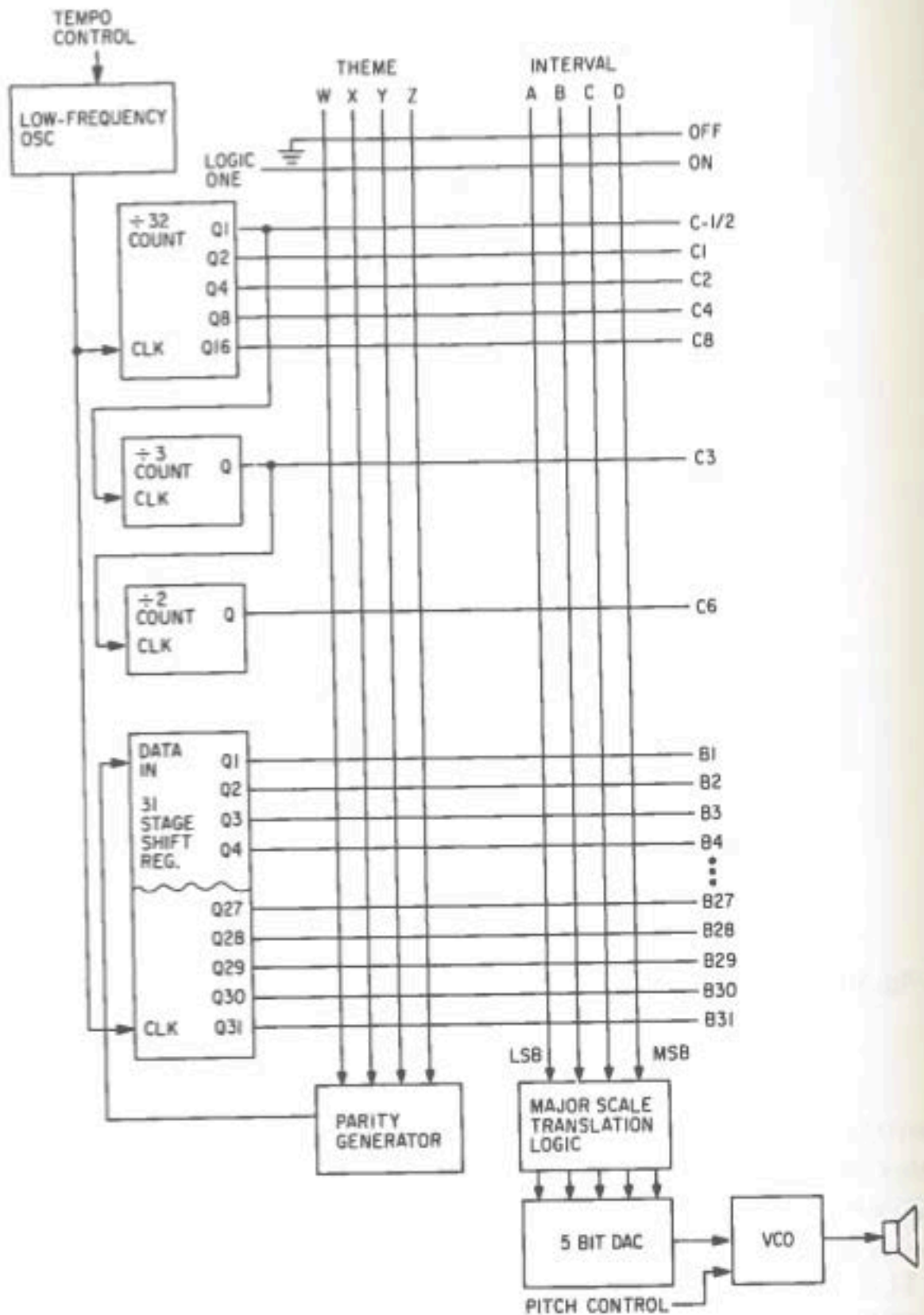
Fig. 10-11. Block diagram of Muse
