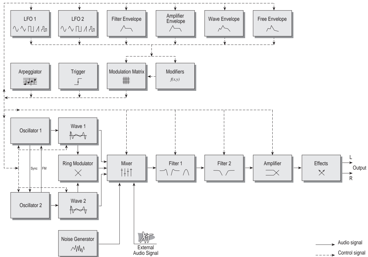
Diagram 3: Block schematic diagram for single sounds
