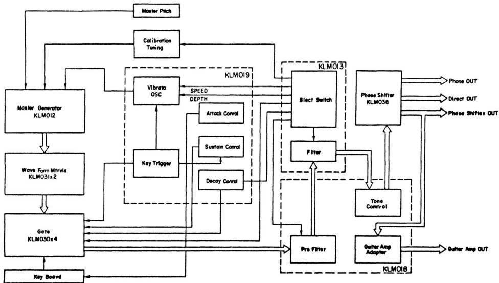
Block Diagram
