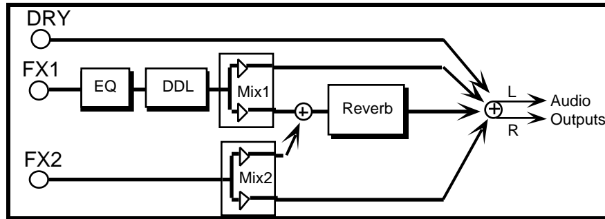
EQ-DDL+REVERB Routing
