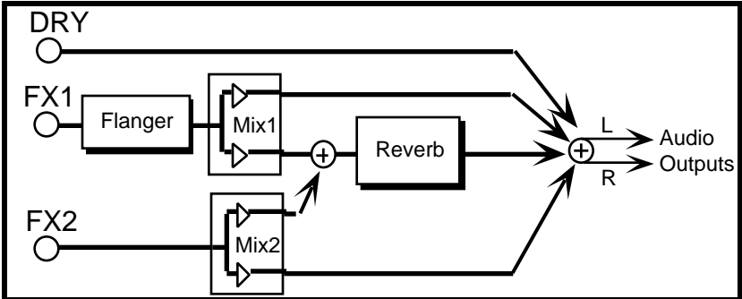
FLANGER+REVERB Routing
